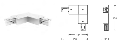
WLLC-RT
